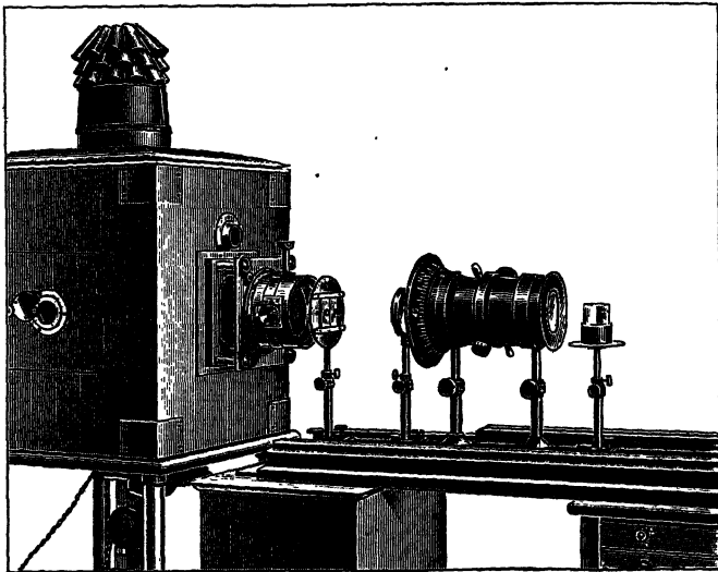
FIG. 109.—Experiment to show Rectangular Polarisation of the two Spectra afforded by a 60^\circ -Prism of a Doubly Refracting Crystal cut to afford two Indices of Refraction.
